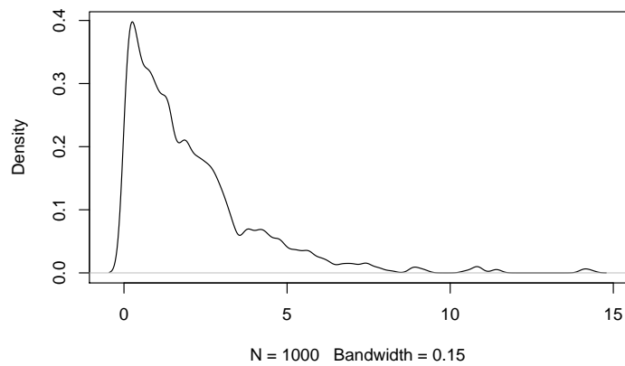
density.default(x = distribution_gamma, bw = bande_passante_gamn
